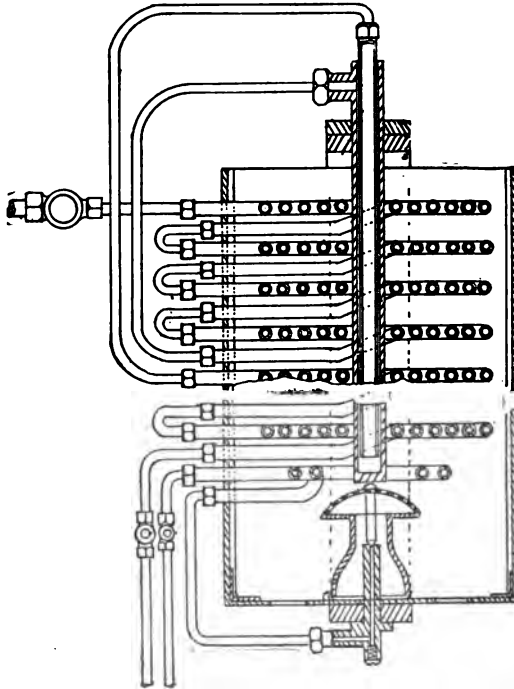
FIG. 180.—Sectional Elevation of the Blaxton Flash Generator.
